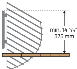
Figure 6. Installing HUUM DROP electric heater inside the sauna bench
