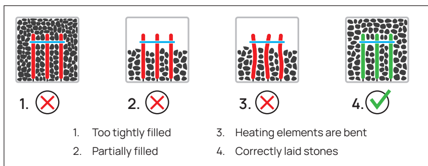
Figure 7. Placing the stones in DROP 4 and DROP 6 with 3 heating elements
