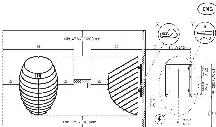
Figure 1. Positioning of the heater
