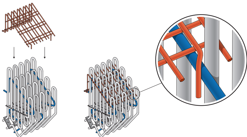
Figure 5. Installation of the retainer of HUUM DROP 7 and DROP 9 with 5 heating elements.
