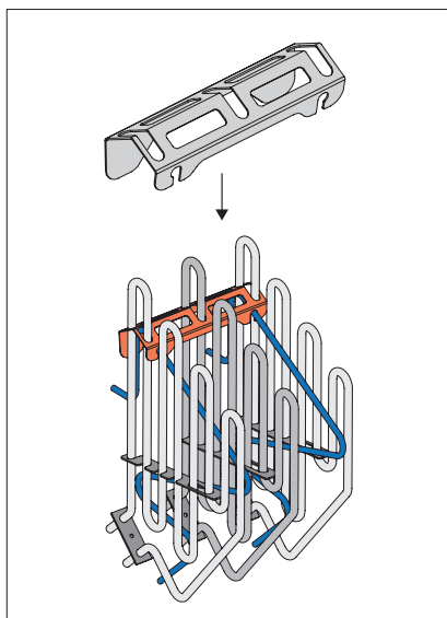
Figure 3. Installation of the retainer of HUUM DROP 4 and 6 with 3 heating elements.
