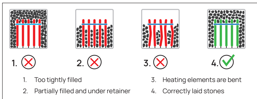
Figure 8. Placing the stones in DROP 7 and DROP 9 with 5 heating elements.
