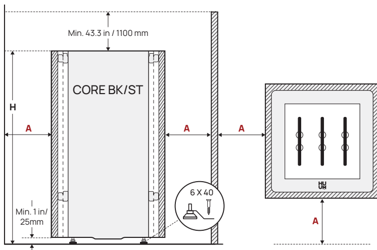
Figure 2. Positioning of the CORE BK/ST electrical heater.
